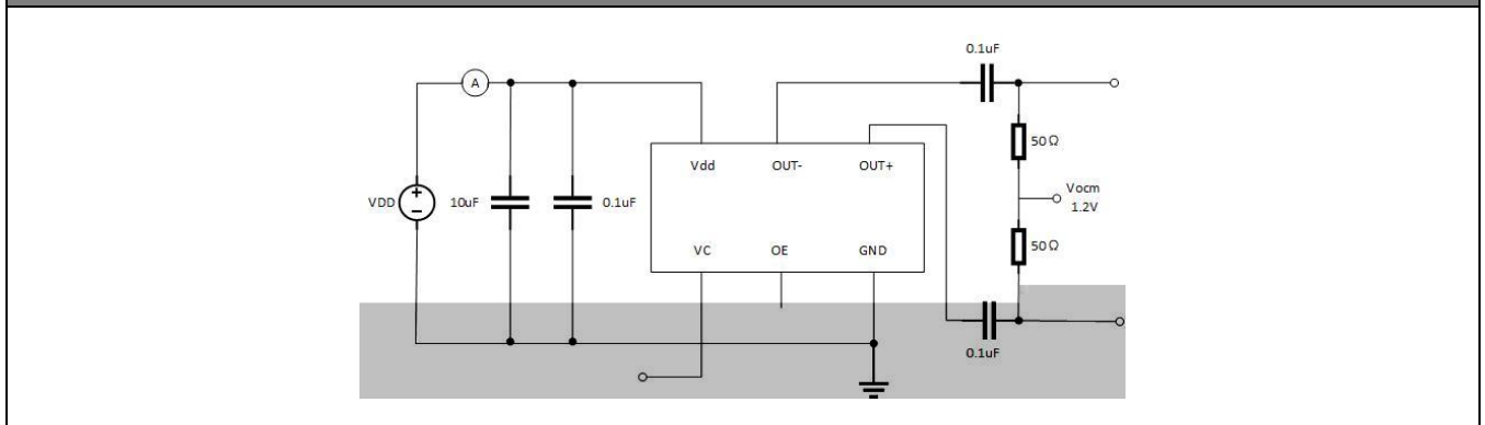
LVDS Test Circuits for 1.8V only
